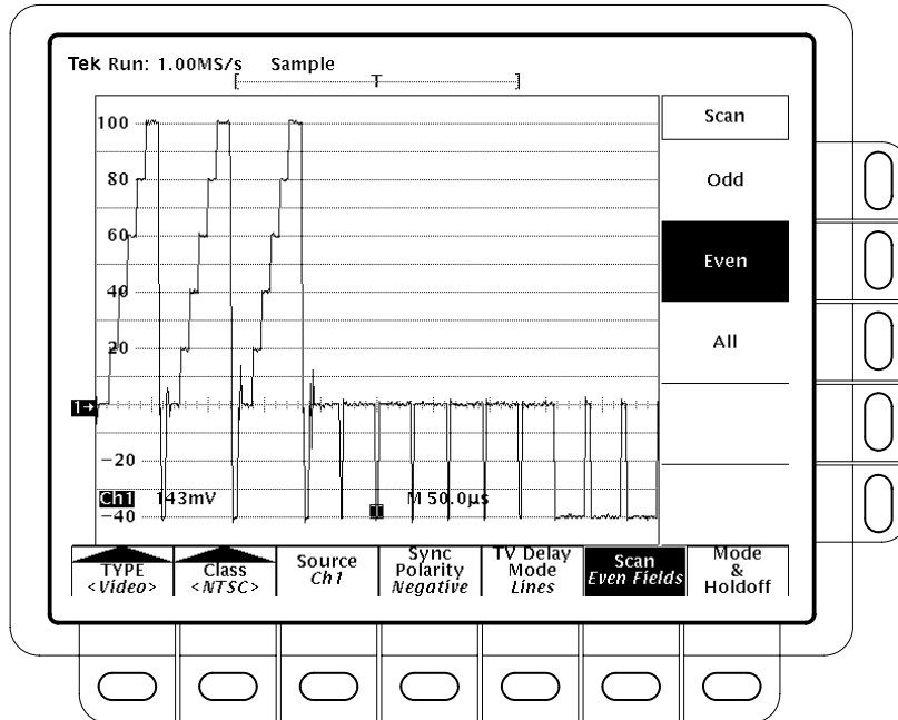
Figure 3–71: Video Trigger — Scan Parameter
